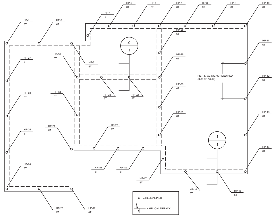
HELICAL PIER FOUNDATION PLAN NO SCALE
