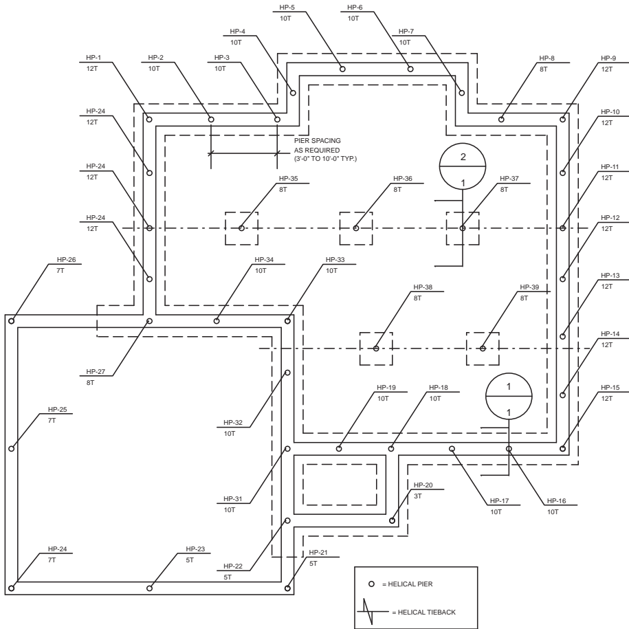
HELICAL PIER FOUNDATION PLAN NO SCALE
