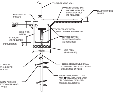
1 EXTERIOR FOUNDATION DETAIL NO SCALE
