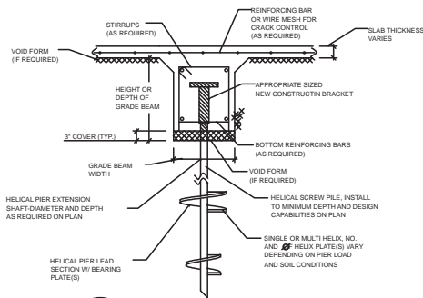
2 INTERIOR GRADE BEAM DETAIL NO SCALE
