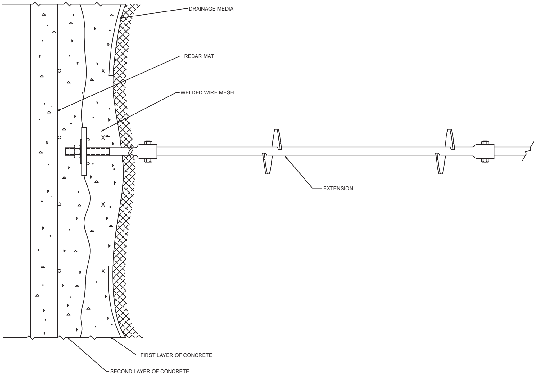
TYPICAL PLAN VIEW OF PERMANENT SOIL SCREW RETENTION WALL SYSTEM, WALL SECTION
